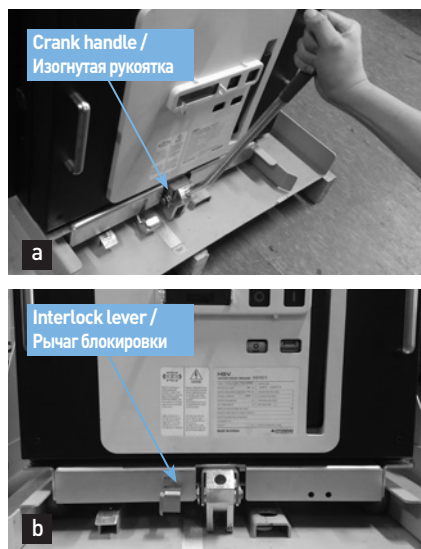
Fig. 4-6 Insertion of the E/F Type (2) /
