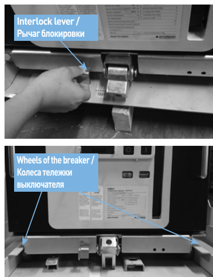
Fig. 4-5 Insertion of the E/F Type (1) /
