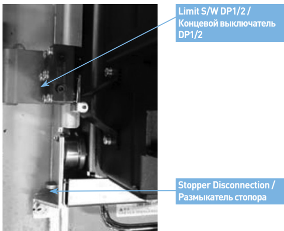
Fig. 4-11 Insertion of the Motorized Truck Type /
