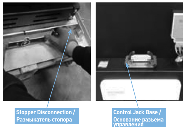
Fig. 4-12 Insertion of the Motorized Truck Type /
