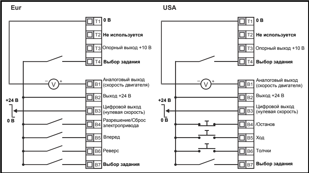
Рис. 10-29 Pr 11.27 = Pr
