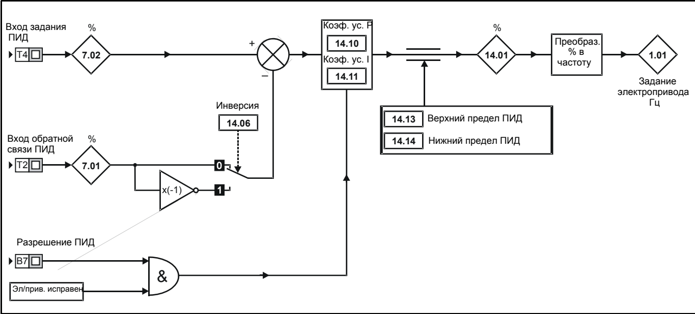
Рис. 10-35 Pr 11.27 = HUAC
