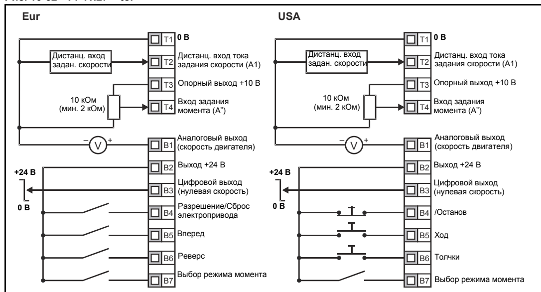
Рис. 10-32 Pr 11.27 = tor
