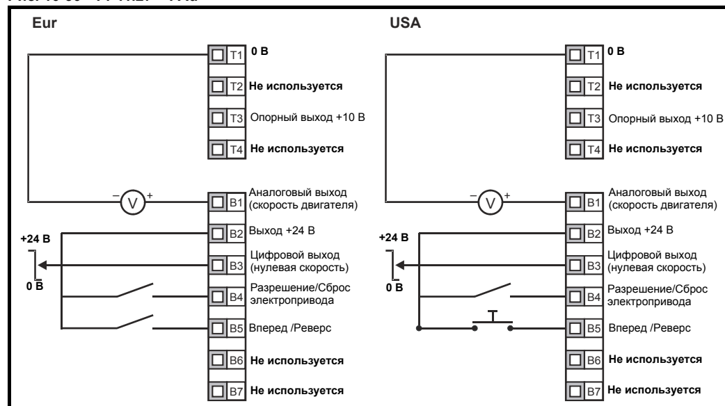
Рис. 10-30 Pr 11.27 = PAd
