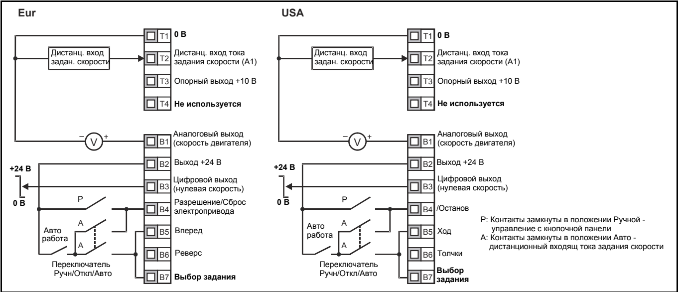
Рис. 10-35 Pr 11.27 = HUAC
