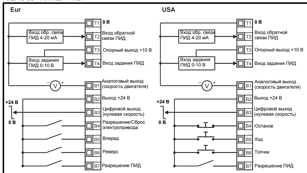
Рис. 10-33 Pr 11.27 = Pid
