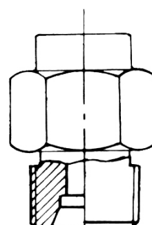
– Raccordo – Fitting
