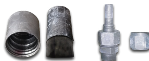
E-Coat 1000 after 1,000 hours ASTM B117 (ISO 9227) salt spray test
