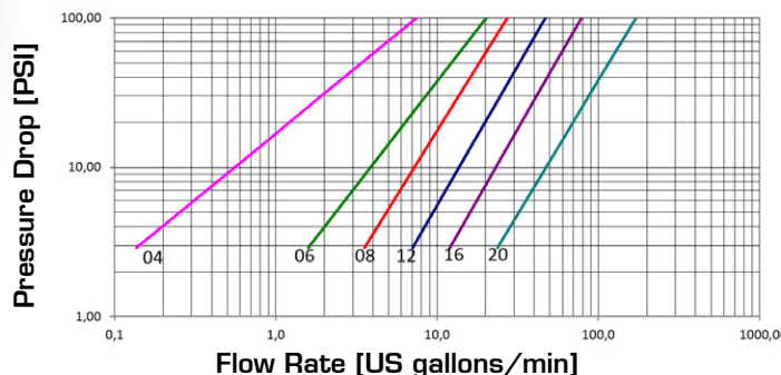
Pressure Drop
