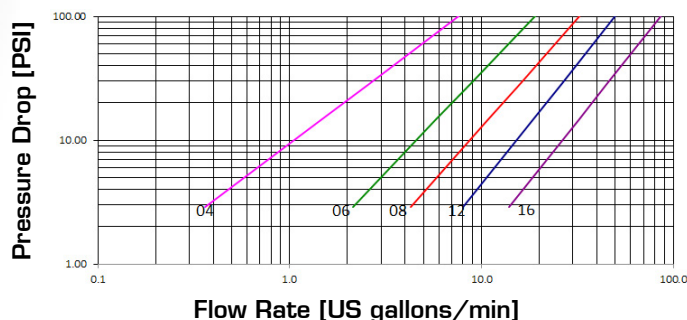
Pressure Drop
