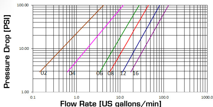
Pressure Drop
