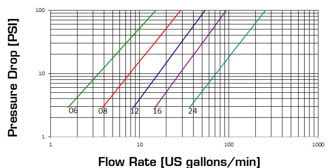
Pressure Drop
