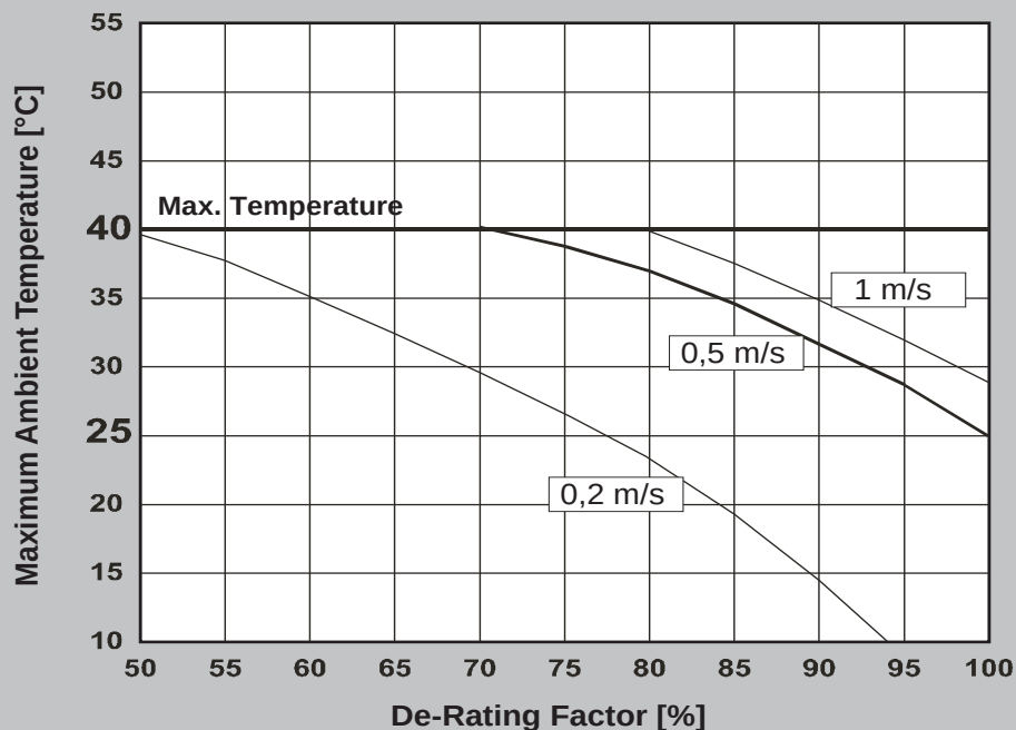
De-Rating of 10" Rewindable Motors with PVC Insulation
