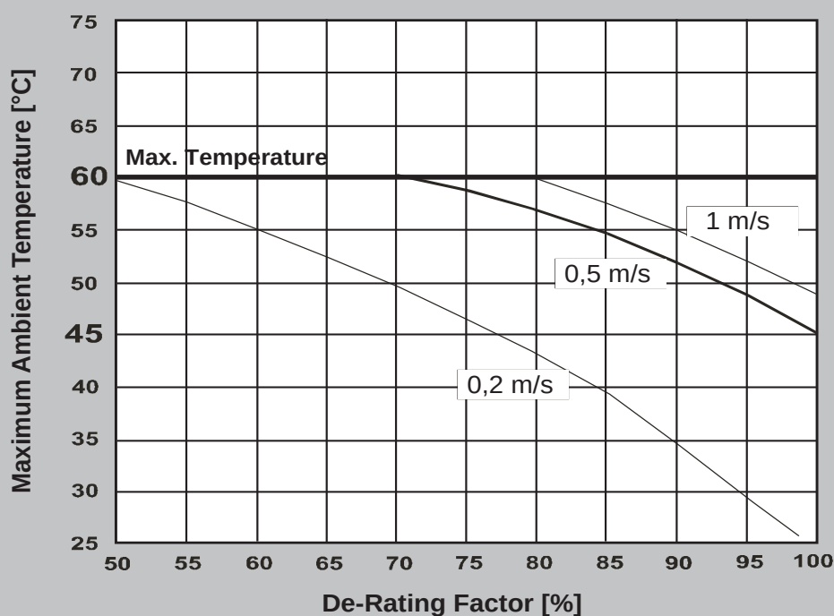
De-Rating of 10" Rewindable Motors with PE2/PA Insulation
